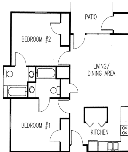
TWO BEDROOM OPTION
